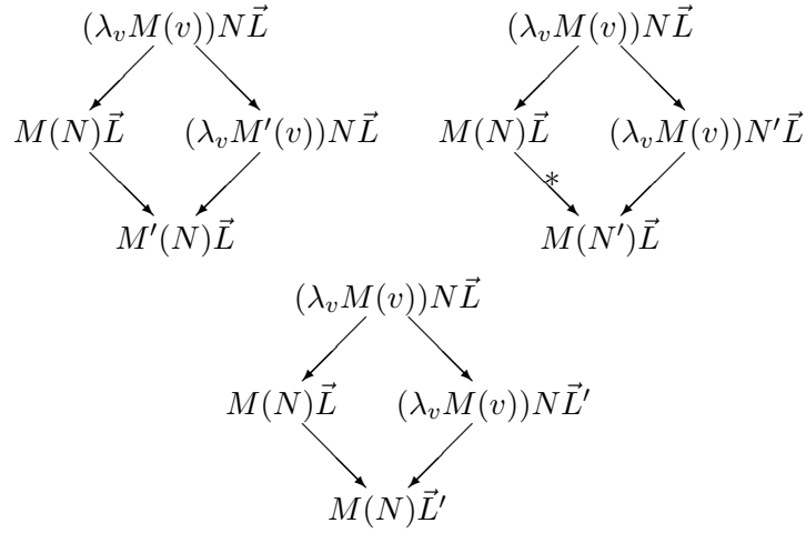
FIGURE 2. Weak confluence of \rightarrow
