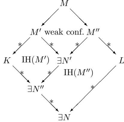
FIGURE 1. Proof of Newman's lemma
